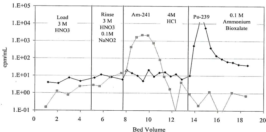
TRU Resin Elution Curve
